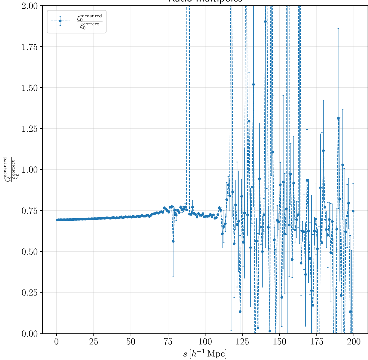
Ratio multipoles
