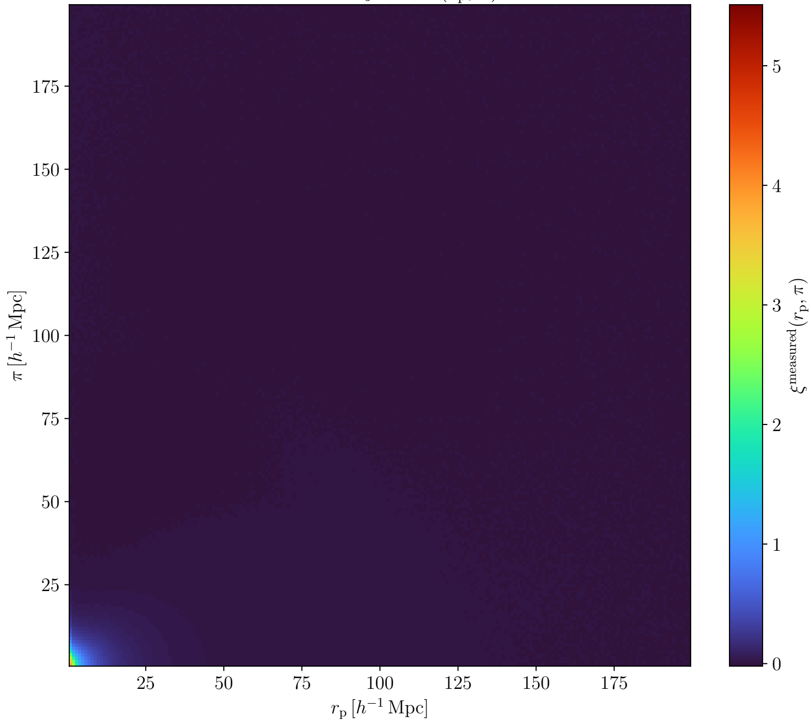
imshow of \xi^{\text{measured}}(r_p, \pi)
