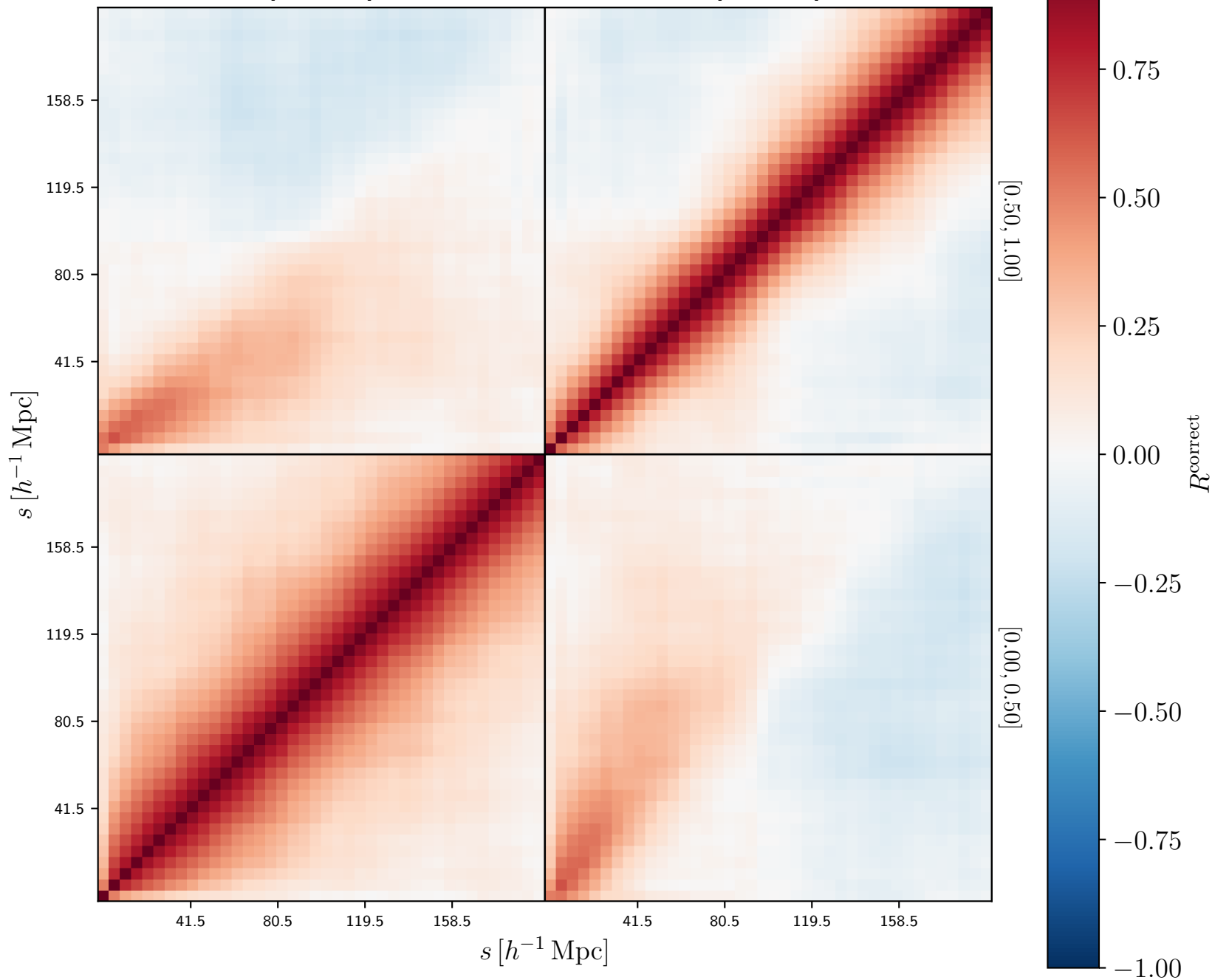
Correlation Matrix for \xi_{[\mu_{\min}, \mu_{\max}]} correct [0.00, 0.50] [0.50, 1.00]
