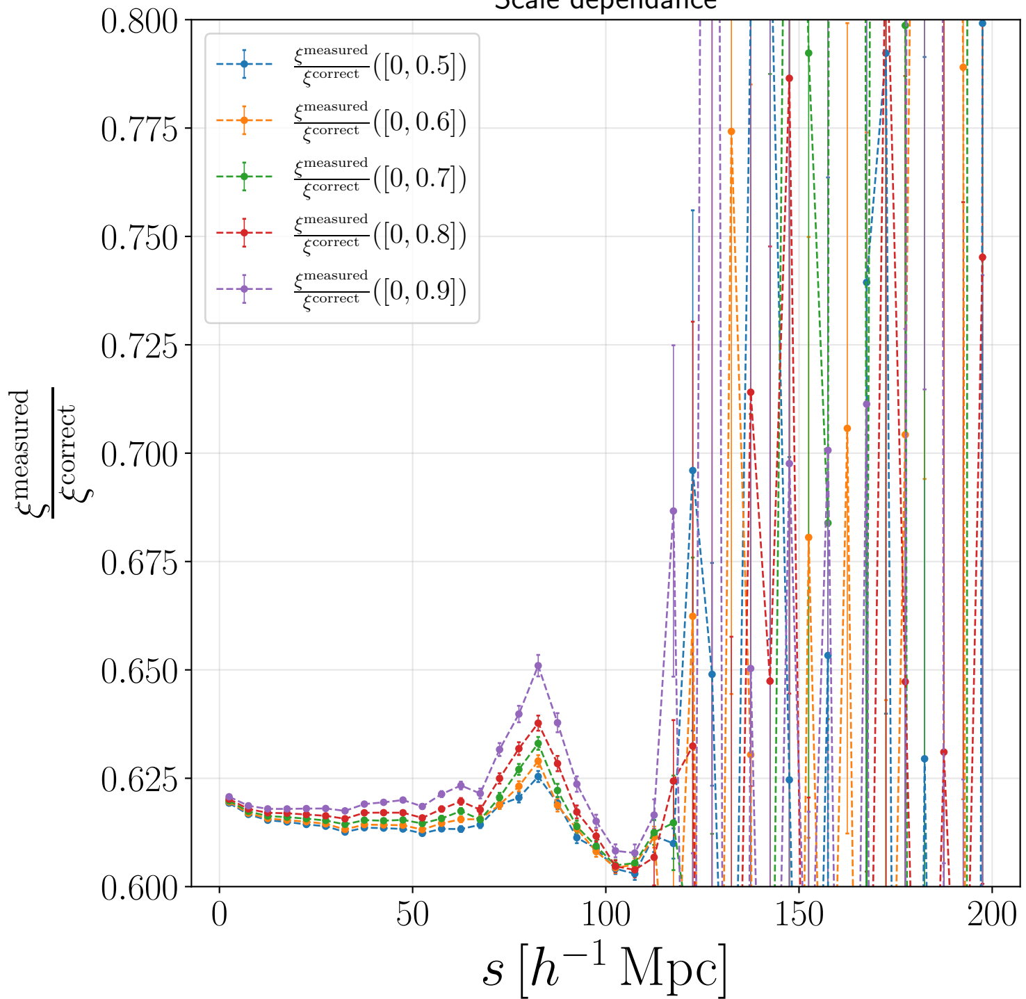
Scale dependance
