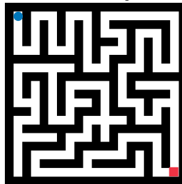
Backtracking
