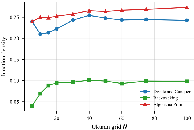
(a) Junction density = junctions / N^2
