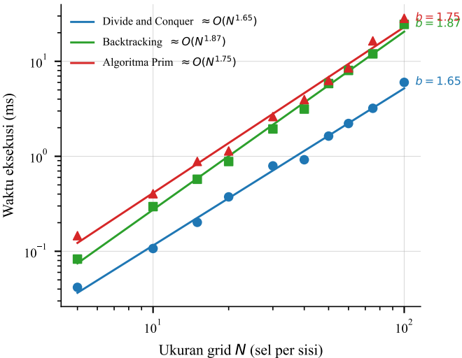
Time complexity: power-law fit ( t = aN^b )
