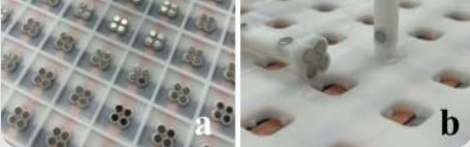
(a) Array of Magnets on the Bottom of the XY-Axis Two-Dimensional Plane; (b) Magnetic Groups on the Base of the Z-Axis Rod
