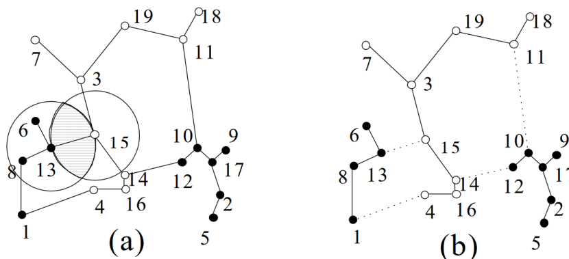
Figure 1: An visualization of the RNG for a binary classification problem represented by black and white points. (a) An example of a 2D RNG graph construction. (b) Identifying cut edges with dotted lines.
