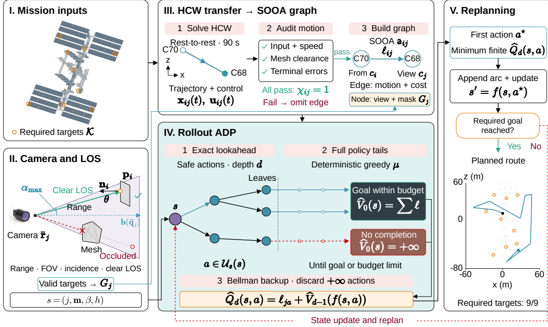
Fig. 1. Viability-preserving rollout ADP for orbital inspection. I. International Space Station (ISS) mesh and required targets \mathcal{K} . II. Camera-valid targets G_j from range, field of view (FOV), incidence \theta \leq \theta_{\max} , and line of sight (LOS) checks. III. HCW transfer, motion audits, and directed SOOA construction; C70 and C68 are archived candidate IDs. IV. Depth- d Bellman lookahead with complete greedy base-policy tails. At each leaf, \sum \ell denotes the full tail cost; +\infty denotes no certified completion within the remaining budget. V. First-action selection and planning-state updates toward completion of all required targets. The tree is schematic; the 9/9 route is an archived offline plan. ISS geometry: National Aeronautics and Space Administration (NASA), NASA .
