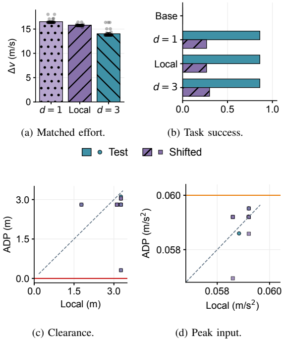
Fig. 5. Nine-target component and safety comparison. Base is the task-aware incumbent; d = 1, 3 are ADP depths; Local is ADP-seeded local search. (a) Physical \Delta v over 43 jointly completed test cases. (b) All-required success. (c) Minimum clearance above the safety margin. (d) Peak input, with the 0.060 m/s 2 limit in orange.
