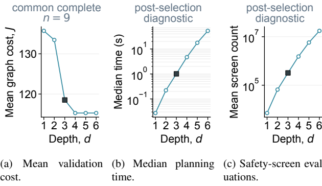
Fig. 3. Post-selection depth diagnostic on 12 validation cases. The square marks the primary depth-three setting; cost uses the nine cases completed at every depth, and panels (b), (c) use logarithmic scales.
