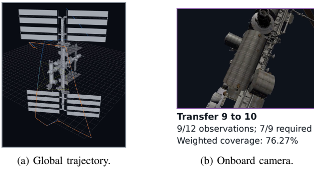
Fig. 8. RViz display: (a) planned (blue) and executed (orange) trajectories with camera FOV (yellow); (b) onboard Gazebo camera. Crops from one frame during transfer 9–10.
