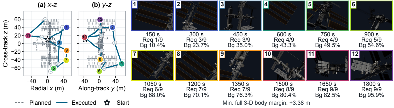
Fig. 7. Twelve-view ROS 2 execution with 90 s transfers and 60 s settling intervals. Panels (a), (b) highlight odd and even observations at equal scale; the camera rows show all accepted views with mission time, required targets (Req), and weighted coverage (Bg). The run accepts 9/9 required targets and 95.86% background coverage while maintaining the full-mesh safety margin.
