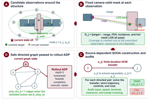
Fig. 1. OrbInspect formulation and data flow. (a) Candidate observations are generated around an ISS-scale structure outside the full-mesh safety margin. (b) Range, field of view, incidence, and full-mesh line of sight define the fixed visible-target mask G_j at each prescribed observation. (c) Each ordered node pair is assigned a separately solved finite-duration HCW transfer; its trajectory, controls, cost, sampled constraints, and swept-mesh crossing test determine the directed-edge indicator \chi_{ij} . (d) Edges with \chi_{ij} = 1 form the safe directed SOOA graph whose shield-admissible actions are passed to the rollout-ADP policy in Fig. 2.
