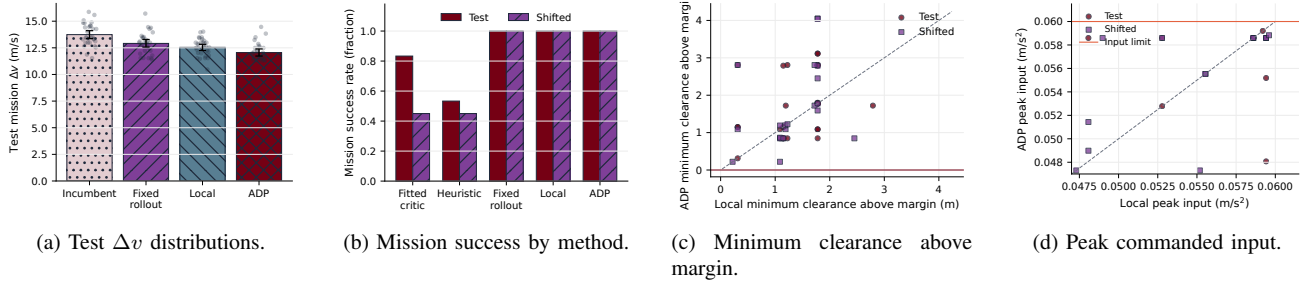
Fig. 5. Component and safety audit. Bootstrap intervals accompany the method means in (a). Panel (b) exposes the failure of standalone fitted and hand-scaled critics; fixed rollout, local search, and proposed adaptive rollout reach every goal. Panels (c) and (d) compare the common sampled shield margins, with horizontal colored lines denoting acceptance limits. Passive drift and uncertainty are not evaluated.
