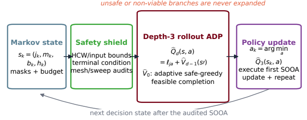
Fig. 2. Proposed viability-preserving rollout ADP. The finite candidate-graph state carries current node, covered and selected masks, and remaining budget. The safety shield removes inadmissible SOOAs before search. A depth- d exact prefix is terminated by a complete adaptive safe-greedy simulation; a branch is viable only if this completion reaches the coverage goal. The first minimizing action is executed and the value is recomputed.
