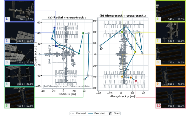
Fig. 7. Trajectory-linked camera views from the accepted corrected validation_002 task. Views 1–5 link locally to the radial-cross-track ( x – z ) projection, and views 6–10 link to the along-track-cross-track ( y – z ) projection; hollow gray markers retain the other observations as context. Inset labels give mission time and cumulative coverage. Dashed gray and solid blue denote planned and executed paths, and the star is the initial state. Apparent overlap in either projection does not imply contact: the annotated clearances and collision decision use the full 3-D transformed mesh and swept path. Gazebo rendered the views, while ROS HCW dynamics propagated state; coverage came from frozen geometric visibility masks, not image pixels.
