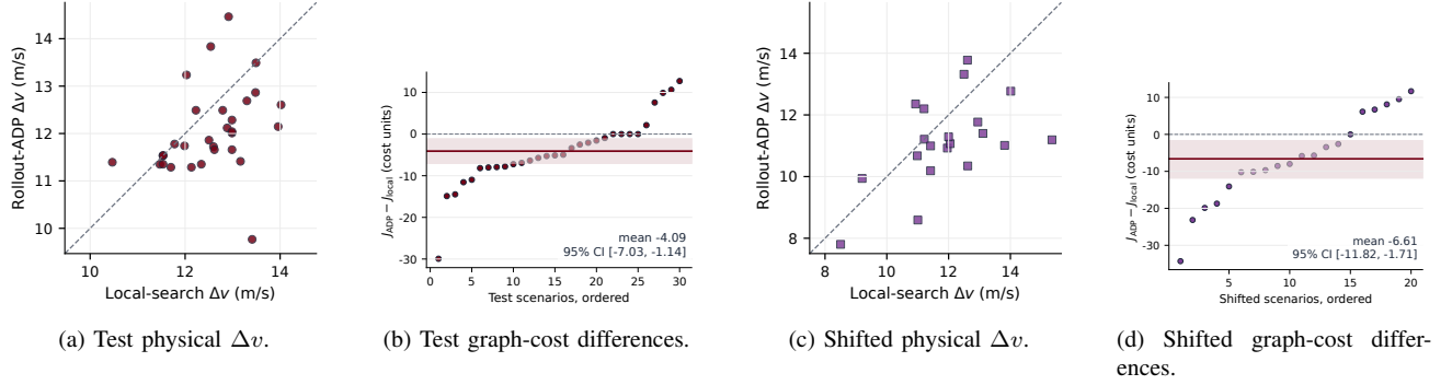
Fig. 4. Held-out paired performance of proposed rollout ADP versus audited local search. Dashed lines denote parity. Rollout ADP wins 21 of 30 test pairs with four numerical ties and wins 14 of 20 shifted pairs with one tie. The shaded bands and horizontal lines in (b) and (d) report paired-bootstrap intervals and mean differences; coverage success is matched in every panel.
