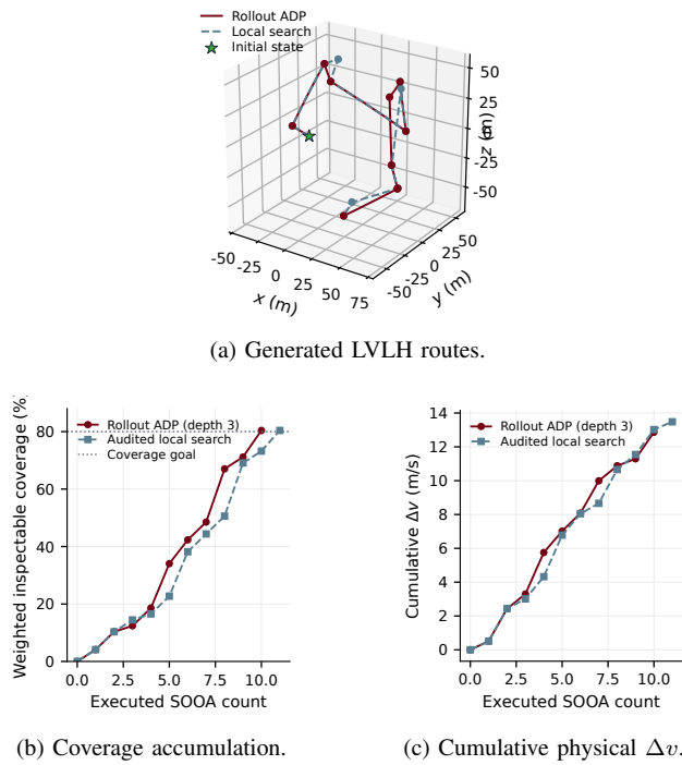
Fig. 6. Illustrative median-effect held-out case. Markers in (a) are terminal observations and the star is the common initial state. The ADP route reaches the coverage goal after 10 actions; local search uses 11. The selection is post hoc and does not replace the all-scenario inference.
