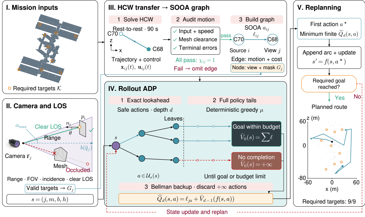
Fig. 1. Viability-preserving rollout ADP for orbital inspection. I. ISS mesh and required targets \mathcal{K} (orange rings). II. Camera-valid targets G_j from range, FOV, incidence \theta \leq \theta_{\max} , and LOS checks. III. HCW transfer, motion audits, and directed SOOA construction; C70 and C68 are archived candidate IDs. IV. Depth- d Bellman lookahead with complete greedy base-policy tails. At each leaf, \sum \ell denotes the full tail cost; +\infty denotes no certified completion within the remaining budget. V. First-action selection and planning-state updates toward the required goal \Gamma_{\mathcal{K}}(m) = 1 . The tree is schematic; the 9/9 route is an archived offline plan. ISS geometry: NASA. Camera photograph: A. Lucke, CC BY-SA 3.0 (illustrative hardware).
