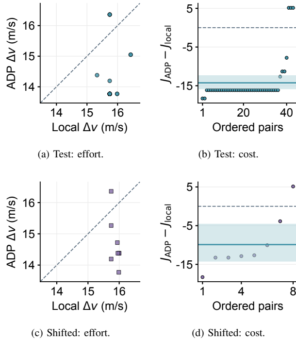
Fig. 4. ADP/seeded-local comparison on jointly completed missions: (a), (b) 43 test pairs; (c), (d) 8 shifted pairs. Panels (a), (c) compare physical \Delta v ; (b), (d) show ordered graph-cost differences in cost units. Dashed lines denote parity. Solid lines and bands give the means and 95% paired-bootstrap intervals: (b) -14.25 [-15.72, -12.46] ; (d) -9.89 [-14.11, -4.69] .
