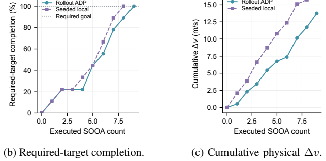
Fig. 6. Representative required-target test pair selected by the median-effect rule. Both methods complete the same required set. Markers identify terminal observations and prescribed samples; the star denotes the common initial state.
