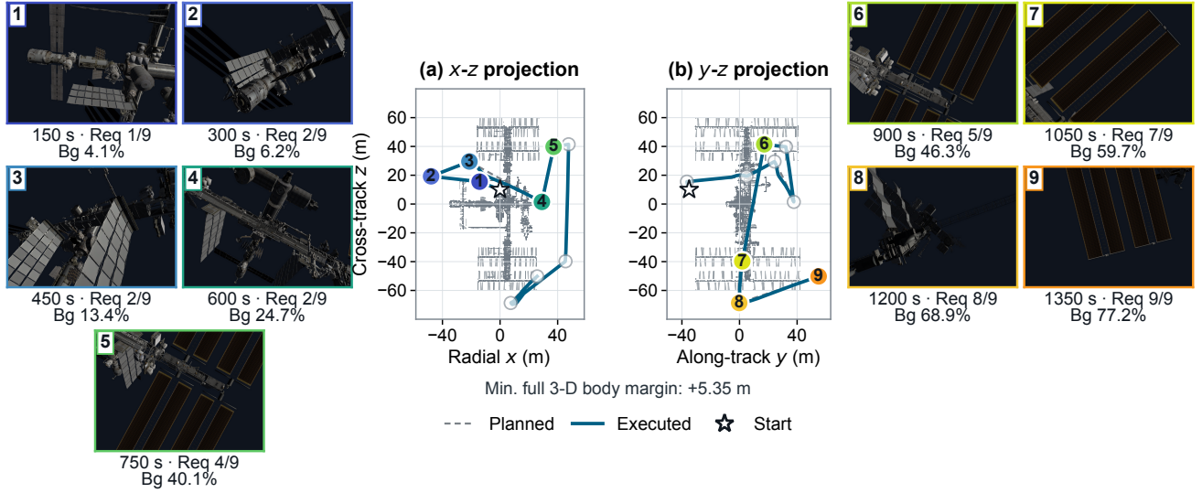
Fig. 7. Required-target ROS 2 execution with 60 s terminal settling after each frozen transfer. All nine observations pass. Matching numbers associate views 1–5 (left) with the x - z projection and views 6–9 (right) with the y - z projection; hollow gray markers retain the other observations. Labels give mission time, accepted required targets (Req), and weighted background coverage (Bg). Dashed gray and solid blue denote the scheduled reference and executed paths; the star marks the initial state. Both projections use the same spatial scale. Uncropped Gazebo frames and trajectory positions come from the same execution. Frozen visibility masks gated by terminal tracking determine target credit. The minimum swept-body margin is audited against the full 3-D mesh.
