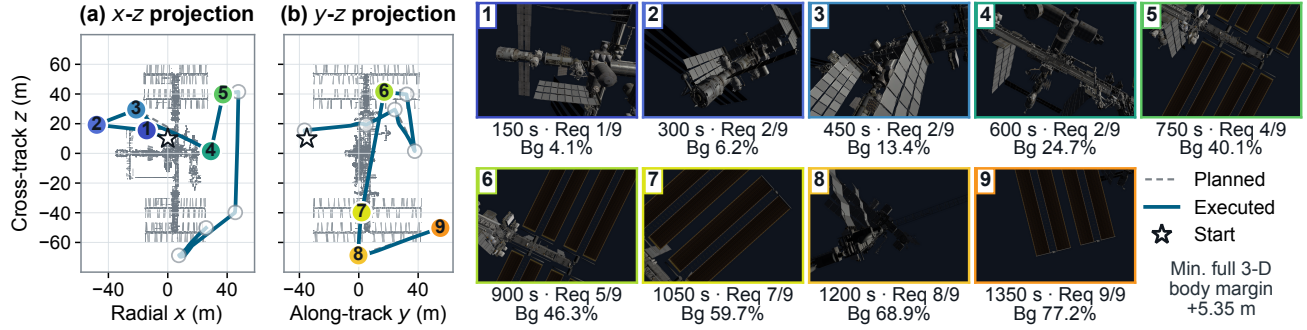
Fig. 7. Required-target ROS 2 execution with 60 s terminal settling after each frozen transfer. All nine observations pass. Numbered markers in (a) and (b) match camera views 1–5 (top row) and 6–9 (bottom row), respectively; hollow gray markers retain the other observations. Both projections use the same spatial scale. Labels give mission time, accepted required targets (Req), and weighted background coverage (Bg). Uncropped Gazebo frames and trajectory positions come from the same execution. Frozen visibility masks gated by terminal tracking determine target credit. The minimum swept-body margin is audited against the full 3-D mesh.
