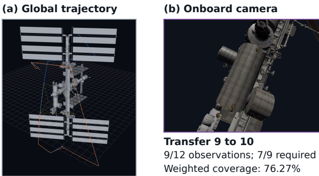
Fig. 8. RViz display: (a) planned (blue) and executed (orange) trajectories with camera field of view (yellow); (b) onboard Gazebo camera. Crops from one frame during transfer 9–10.
