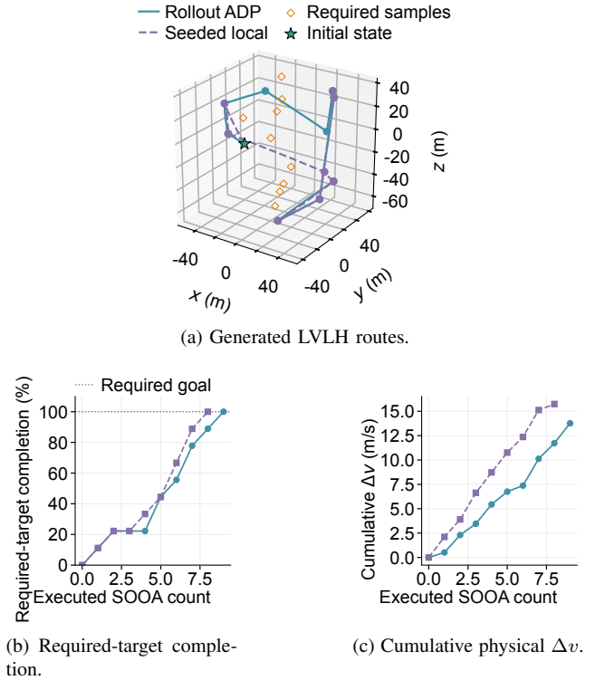
Fig. 5. Representative required-target test pair selected by the median-effect rule. Both methods complete the same required set. Markers identify terminal observations and prescribed samples; the star denotes the common initial state.
