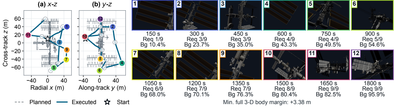
Fig. 6. Twelve-view ROS 2 execution with 90 s transfers and 60 s settling intervals. Panels (a), (b) highlight odd and even observations at equal scale; the camera rows show all accepted views with mission time, required targets (Req), and weighted coverage (Bg). The run accepts 9/9 required targets and 95.86% background coverage while maintaining the full-mesh safety margin.
