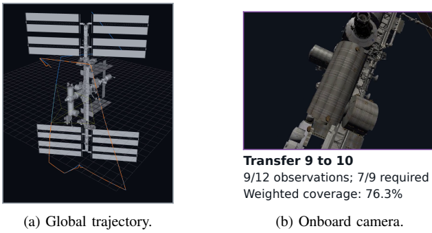
Fig. 7. RViz display: (a) planned (blue) and executed (orange) trajectories with camera FOV (yellow); (b) onboard Gazebo camera. Crops from one frame during transfer 9–10.
