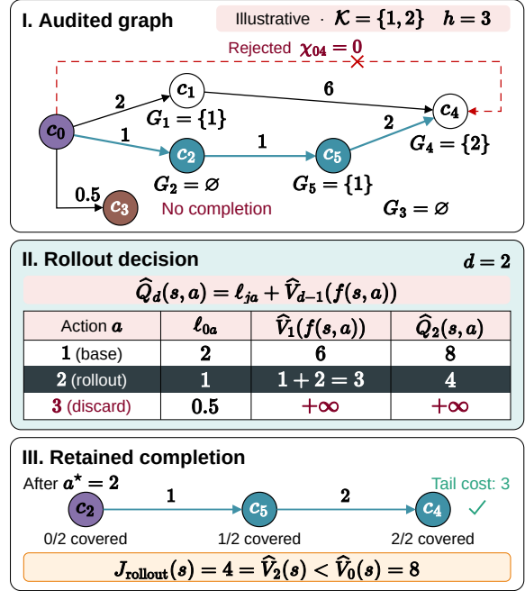
Fig. 2. Illustrative completion-certified rollout ADP, with initial state s = (0, 0, 0, 3) . I. Solid edges are admissible, edge labels are stage costs, and G_j lists visible targets. The dashed transfer is excluded. II. At d = 2 , rollout selects zero-gain connector c_2 for total cost 4, versus base-policy cost 8; action 3 has no certified completion. III. The successor s' = (2, 0, e_2, 2) retains a cost-3 completion. Counts indicate covered required targets; J_{\text{rollout}} is realized graph cost. The example illustrates Propositions 4 and 5. Assigned costs and audit flags are illustrative, not experimental HCW data; the primary study uses d = 3 .
