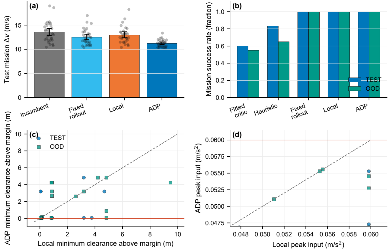
Fig. 6. Component and safety audit. (a) Test \Delta v distributions with bootstrap intervals for method means. (b) Mission success exposes the failure of standalone fitted and hand-scaled critics; fixed rollout, local search, and proposed adaptive rollout reach every goal. (c) Minimum sampled clearance above the 2 m margin and (d) peak input for ADP versus local search. Red lines are acceptance limits. Passive drift and uncertainty are not evaluated.
