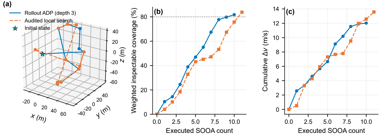
Fig. 7. Illustrative median-effect held-out case. (a) Generated observation-to-observation routes in the LVLH frame; markers are terminal observations and the star is the common initial state. (b) Weighted inspectable coverage versus executed SOOA count. (c) Cumulative physical \Delta v . The ADP route reaches the goal after 10 actions; local search uses 11. The selection is post hoc and does not replace the all-scenario inference.
