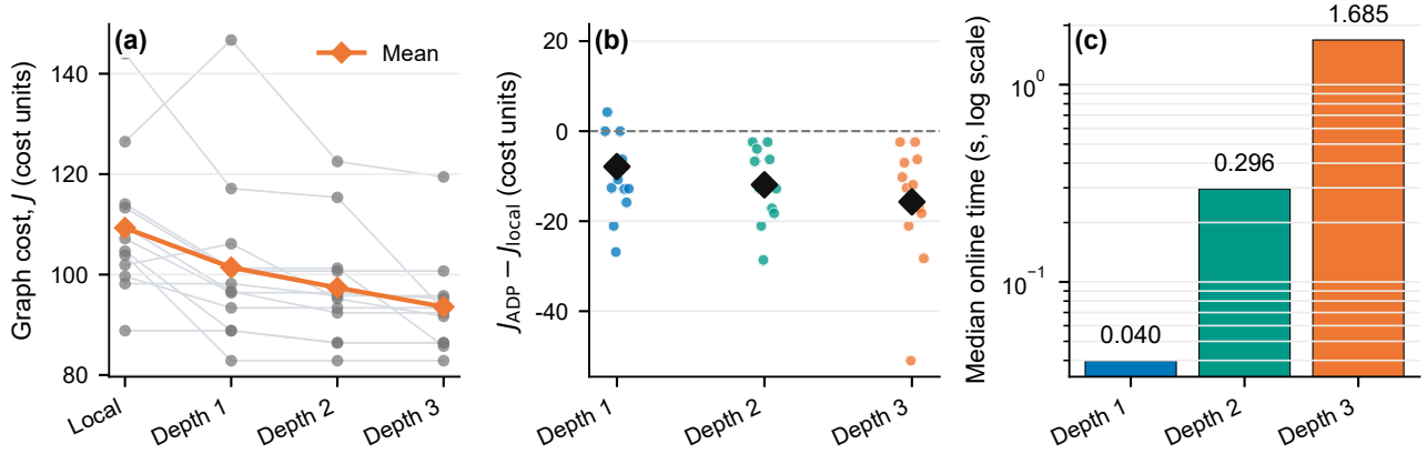
Fig. 3. Validation-only structure selection. All adaptive rollout depths retained mission success; increasing the exact prefix from one to three reduced validation graph cost at increased online computation. Depth three was frozen before held-out evaluation. Validation outcomes are development evidence, not confirmatory test evidence.
