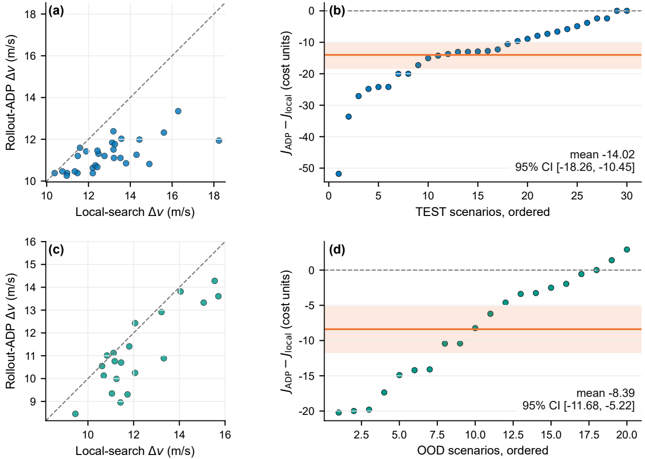
Fig. 5. Held-out paired performance of proposed rollout ADP versus audited local search. (a) Test \Delta v , (b) test graph cost, and (c)–(d) the corresponding shifted-scenario comparisons. Dashed lines denote parity. Rollout ADP wins 28 of 30 test pairs with two numerical ties and wins 17 of 20 shifted pairs with one tie. Insets report paired-bootstrap intervals for the mean difference; coverage success is matched in every panel.
