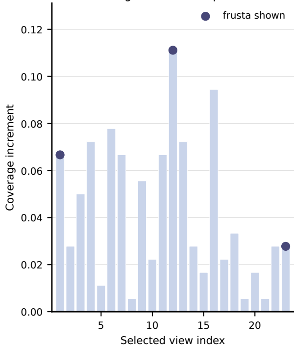
Coverage contribution per view
