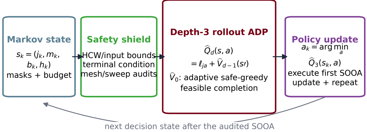
Fig. 2. Proposed viability-preserving rollout ADP. The finite candidate-graph state carries current node, covered and selected masks, and remaining budget. The safety shield removes inadmissible SOOAs before search. A depth- d exact prefix is terminated by a complete adaptive safe-greedy simulation; a branch is viable only if this completion reaches the coverage goal. The first minimizing action is executed and the value is recomputed.
