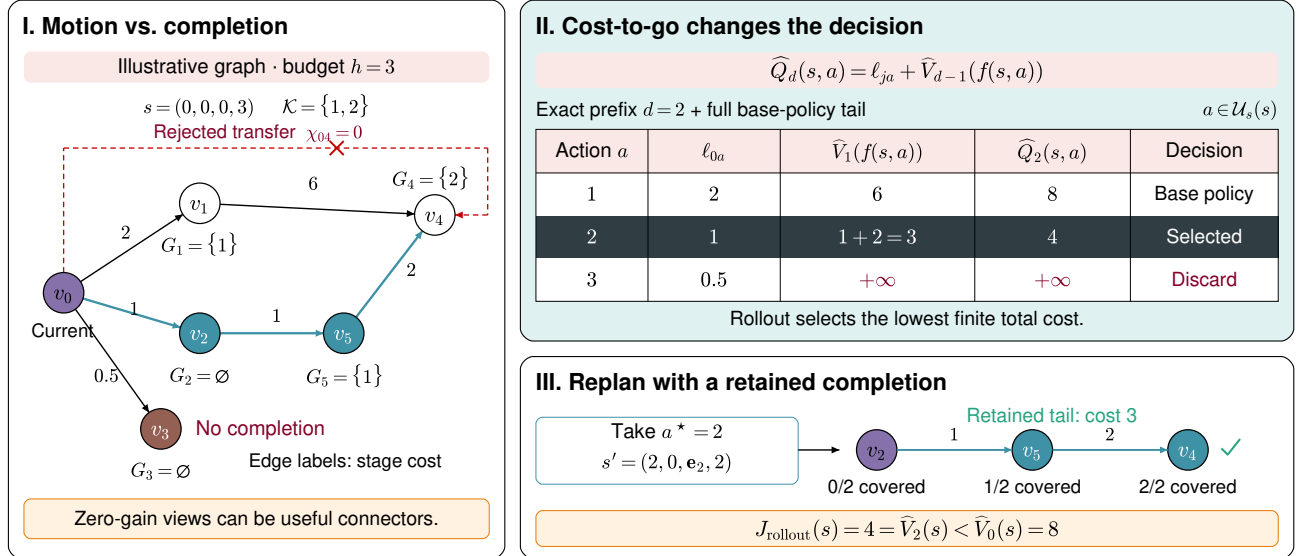
Fig. 2. Completion-certified rollout ADP on an illustrative SOOA graph. I. Required set \mathcal{K} = \{1, 2\} , node visibility sets G_j , and assigned stage costs in arbitrary units. Solid edges pass the assigned audits; the dashed transfer has \chi_{04} = 0 and is excluded. Motion-admissible action 3 has no certified completion, whereas zero-gain view v_2 connects to required observations. II. For s = (0, 0, 0, 3) and illustrative depth d = 2 , the task-aware base policy selects action 1 and completes at cost 8. Rollout selects action 2 and the route 0 \rightarrow 2 \rightarrow 5 \rightarrow 4 at cost 4. III. The successor retains the cost-3 tail 2 \rightarrow 5 \rightarrow 4 ; labels below the nodes count covered required targets. Here J_{\text{rollout}} is the realized graph cost under replanning. The example illustrates Propositions 4 and 5 on a fixed deterministic graph with exhaustive prefixes and a common deterministic base policy. Costs and audit flags are illustrative, not experimental HCW data; the primary study uses d = 3 .
