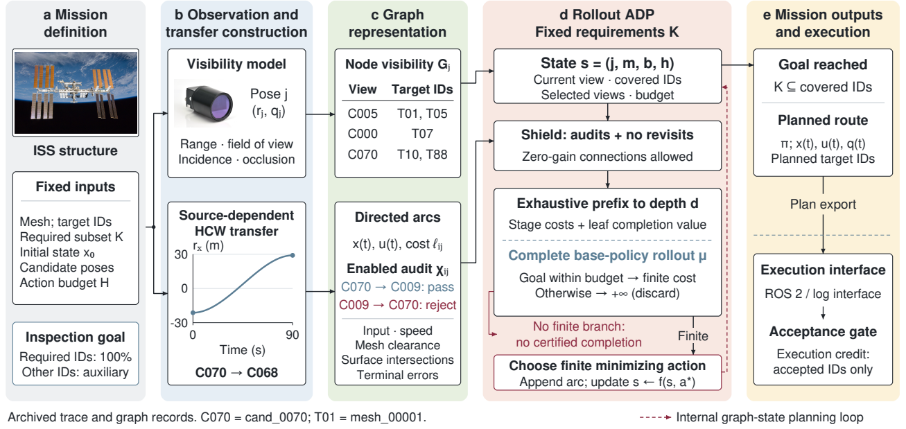
Fig. 1. OrbInspect workflow. (a)–(c) Fixed requirements, camera-valid node masks, and source-dependent audited HCW arcs define the task graph. The transfer trace and indexed records are archived examples; C070 denotes cand_0070 and T01 denotes mesh_00001. (d) Rollout ADP evaluates an exhaustive depth- d prefix with complete base-policy tails, selects a finite minimizing first action, and updates the internal graph state. (e) A goal-reaching plan is exported separately from execution-side observation acceptance. The dashed red arrow is a planning loop, not sensor feedback. Image credits: NASA/STS-132 (ISS); A. Lucke, CC BY-SA 3.0 (camera, illustrative hardware).
