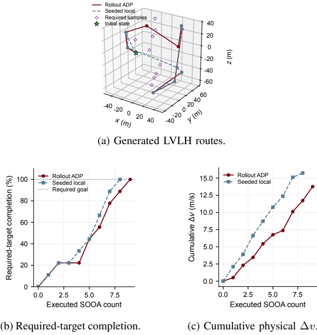
Fig. 6. Representative required-target test pair selected by the median-effect rule. Both methods complete the same required set. Markers identify terminal observations and prescribed samples; the star denotes the common initial state.
