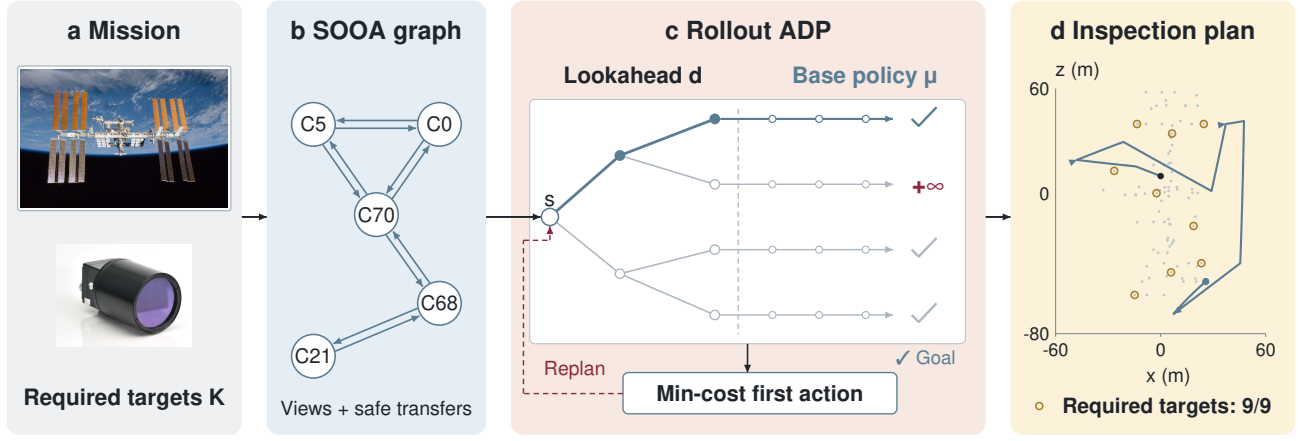
Fig. 1. OrbInspect overview. Audited view-to-view arcs feed rollout ADP, which combines depth- d lookahead with complete base-policy tails and replans after selecting the first action. Check marks denote goal-reaching tails; +\infty denotes noncompletion. The graph (candidate IDs prefixed by C) and planned x - z route are archived examples; gray points are mesh samples and gold rings mark the nine required targets. The tree is schematic, and the route is not an executed result. Image credits: NASA/STS-132 (ISS); A. Lucke, CC BY-SA 3.0 (camera, illustrative hardware).
