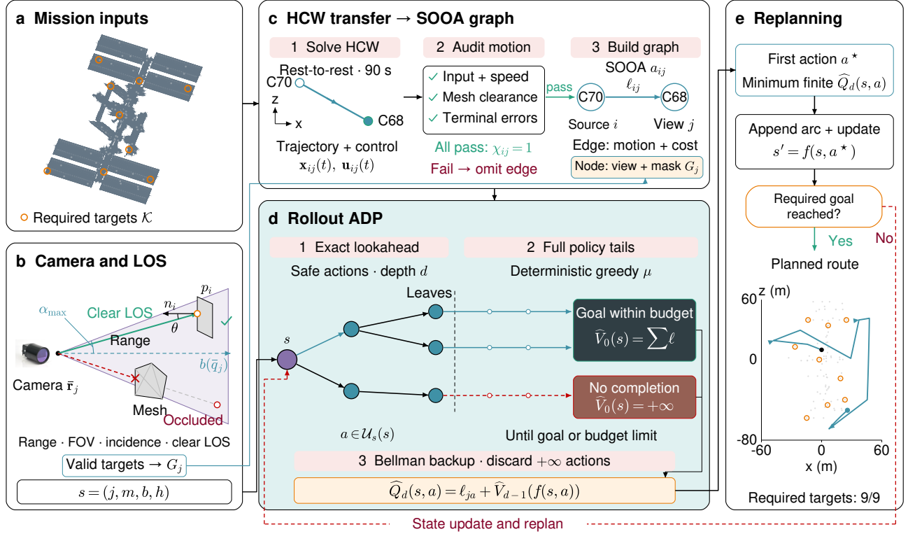
Fig. 1. Viability-preserving rollout ADP for orbital inspection. (a) ISS mesh and required targets \mathcal{K} (orange rings). (b) Camera-valid targets G_j from range, FOV, incidence \theta \leq \theta_{\max} , and LOS checks. (c) HCW transfer, motion audits, and directed SOOA construction; C70 and C68 are archived candidate IDs. (d) Depth- d Bellman lookahead with complete greedy base-policy tails. At each leaf, \sum \ell denotes the full tail cost; +\infty denotes not certified completion within the remaining budget. (e) First-action selection and planning-state updates toward the required goal \Gamma_{\mathcal{K}}(m) = 1 . The tree is schematic; the 9/9 route is an archived offline plan. ISS geometry: NASA. Camera photograph: A. Lucke, CC BY-SA 3.0 (illustrative hardware).
