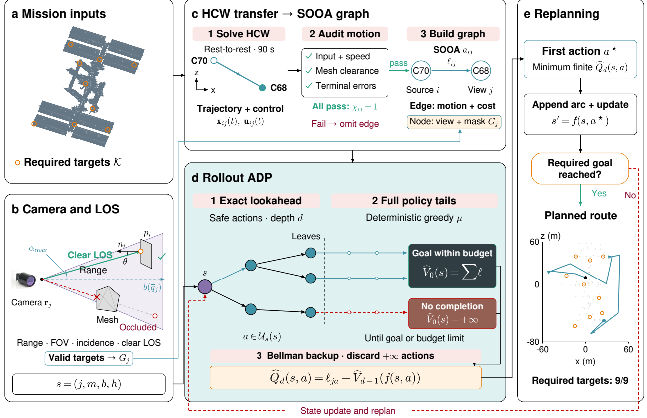
Fig. 1. Viability-preserving rollout ADP for orbital inspection. (a) ISS mesh and required targets \mathcal{K} (orange rings). (b) Camera-valid targets G_j from range, FOV, incidence \theta \leq \theta_{\max} , and LOS checks. (c) HCW transfer, motion audits, and directed SOOA construction; C70 and C68 are archived candidate IDs. (d) Depth- d Bellman lookahead with complete greedy base-policy tails. At each leaf, \sum \ell denotes the full tail cost; +\infty denotes no certified completion within the remaining budget. (e) First-action selection and planning-state updates toward the required goal \Gamma_{\mathcal{K}}(m) = 1 . The tree is schematic; the 9/9 route is an archived offline plan. ISS geometry: NASA. Camera photograph: A. Lucke, CC BY-SA 3.0 (illustrative hardware).
