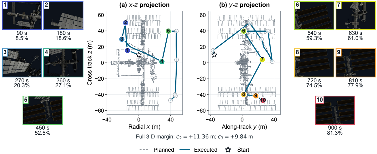
Fig. 7. Historical survey execution: trajectory-linked camera views from the historical ROS 2 validation run with an 80% inspectable-coverage goal. Matching numbers associate views 1–5 (left) with the radial–cross-track ( x – z ) projection and views 6–10 (right) with the along-track–cross-track ( y – z ) projection; hollow gray markers retain the other observations as context. Labels below the images give mission time and cumulative coverage. Dashed gray and solid blue denote planned and executed paths, and the star is the initial state. Clearance is evaluated against the full 3-D mesh and swept path. Gazebo renders the views, ROS HCW dynamics propagate state, and frozen geometric visibility masks determine credited coverage.
