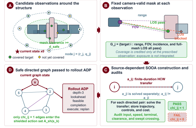
Fig. 1. OrbInspect formulation and data flow. (a) Candidate observations are generated around an International Space Station-scale structure outside the full-mesh safety margin. (b) Range, field of view, incidence, and full-mesh line of sight define the fixed visible-target mask G_j at each prescribed observation. (c) Each ordered node pair is assigned a separately solved finite-duration HCW transfer; its trajectory, controls, cost, sampled constraints, and swept-mesh crossing test determine the directed-edge indicator \chi_{ij} . (d) Edges with \chi_{ij} = 1 form the safe directed SOOA graph whose shield-admissible actions are passed to the rollout-ADP policy in Fig. 2.
