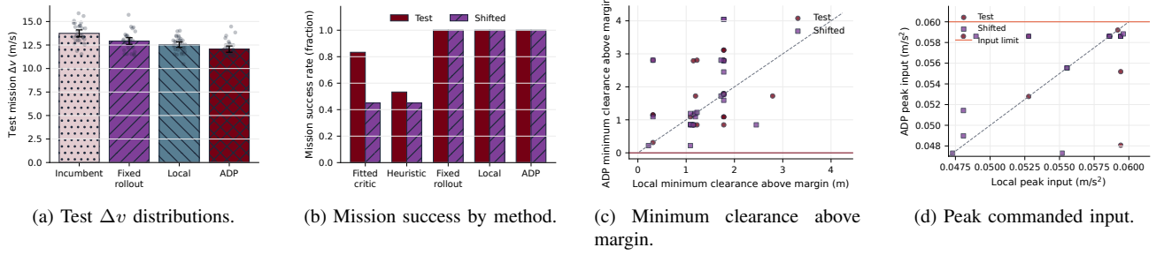
Fig. 5. Component and safety audit. Bootstrap intervals accompany the method means in (a). Panel (b) exposes the failure of standalone fitted and hand-scaled critics; fixed rollout, local search, and proposed adaptive rollout reach every goal. Panels (c) and (d) compare the common sampled shield margins, with horizontal colored lines denoting acceptance limits. Passive drift and uncertainty are not evaluated.
