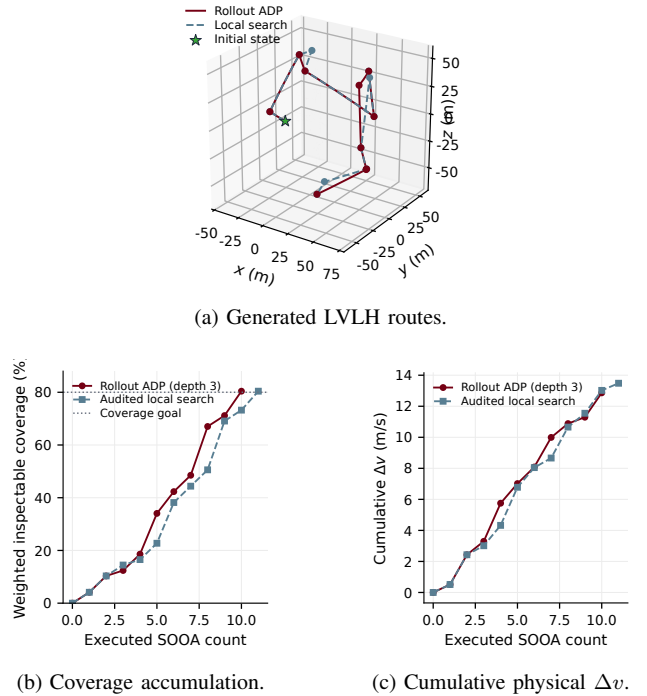
Fig. 6. Illustrative median-effect test case. Markers in (a) are terminal observations and the star is the common initial state. The ADP route reaches the coverage goal after 10 actions; local search uses 11. The selection is post hoc and does not replace the all-scenario comparison.
