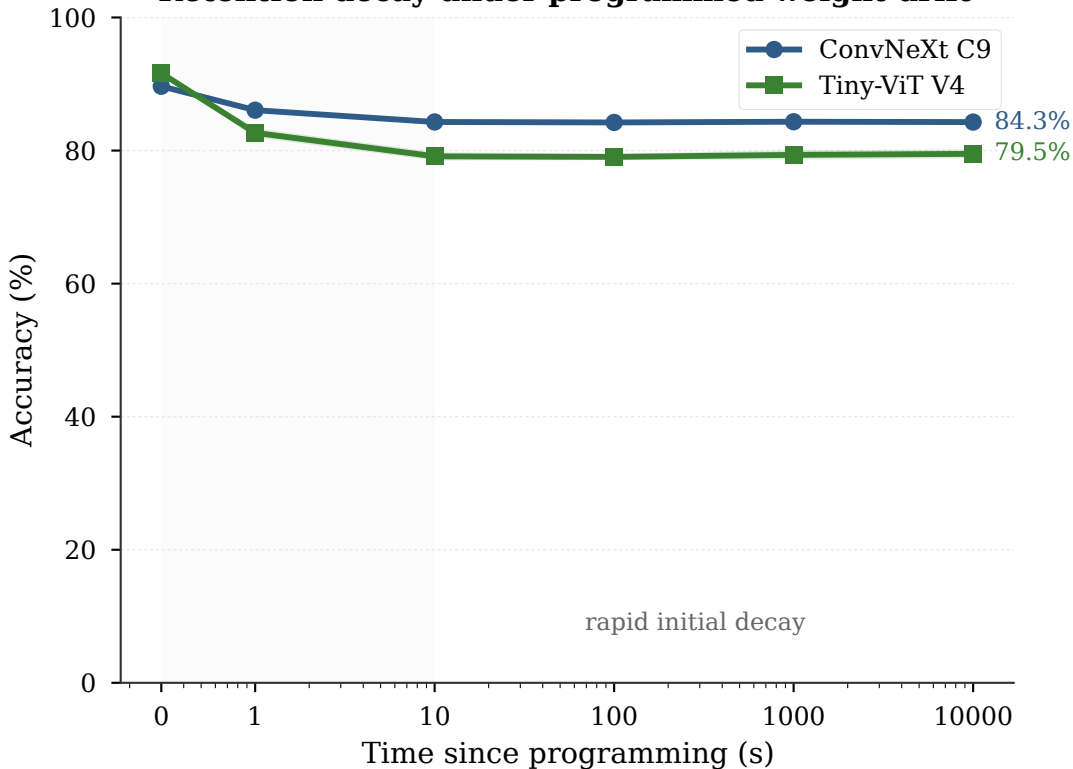
Retention decay under programmed weight drift
