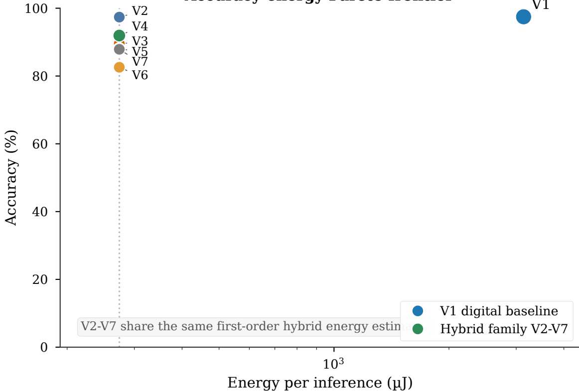
Accuracy-energy Pareto frontier
