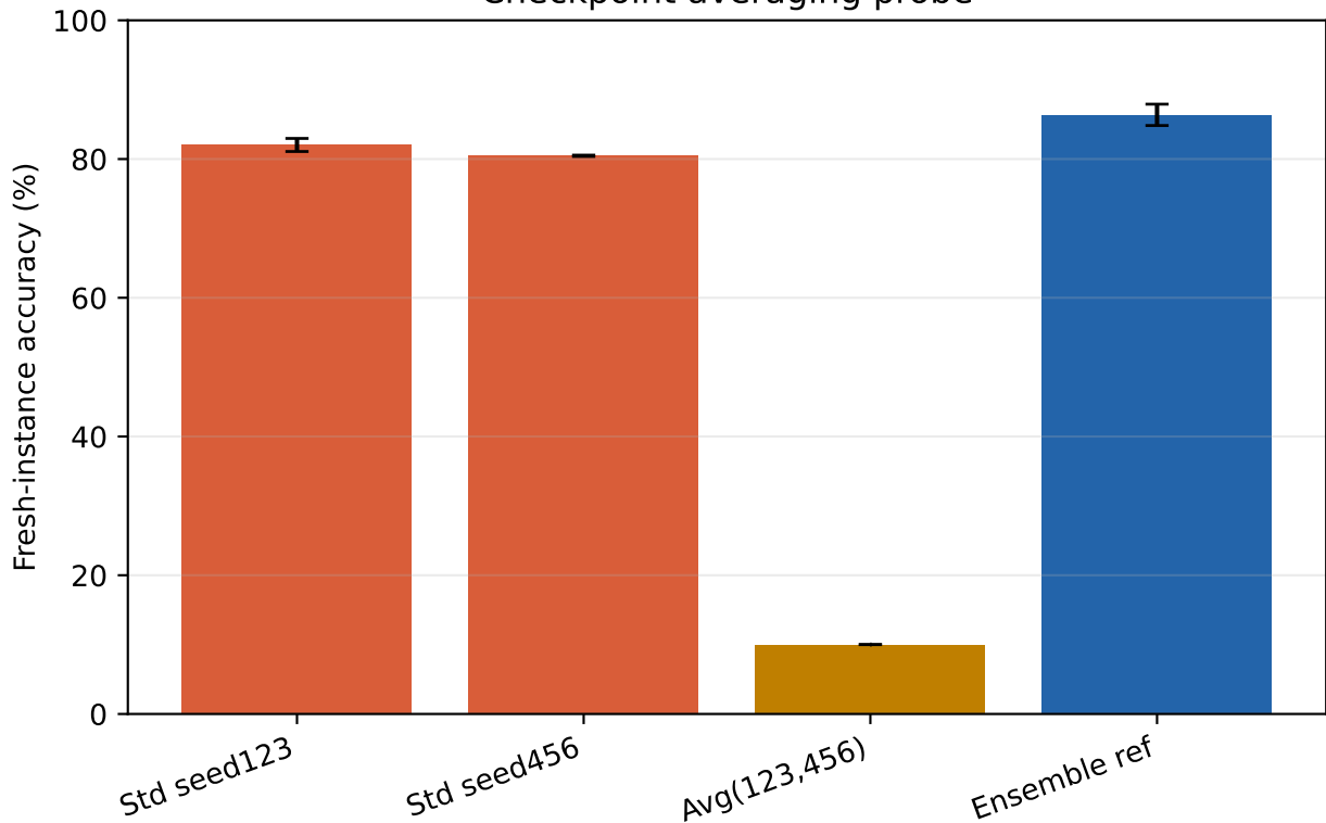
Checkpoint averaging probe
