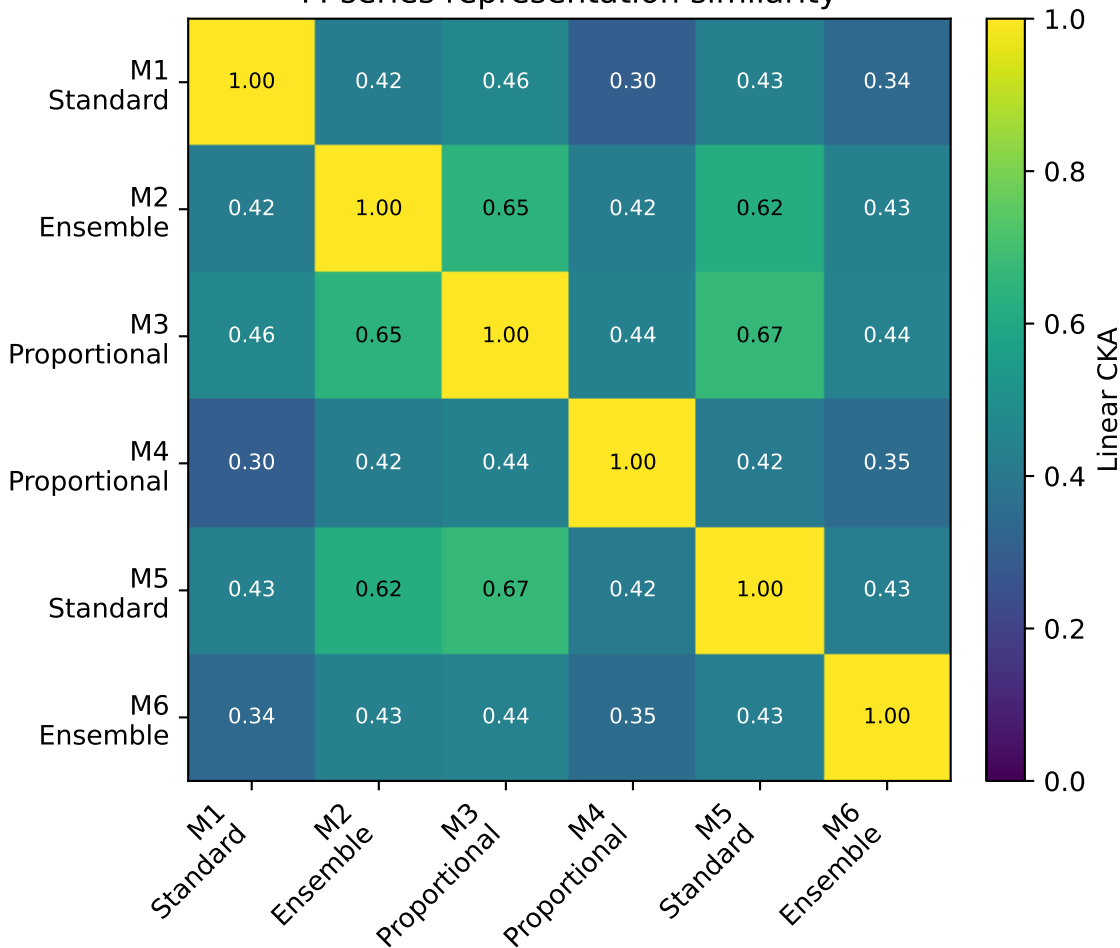
M-series representation similarity
