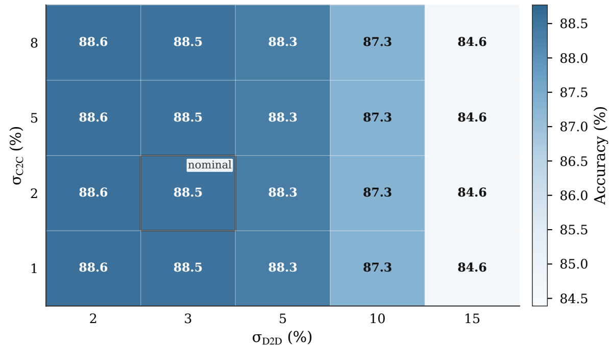
Zhang-proxy C2C/D2D sensitivity
