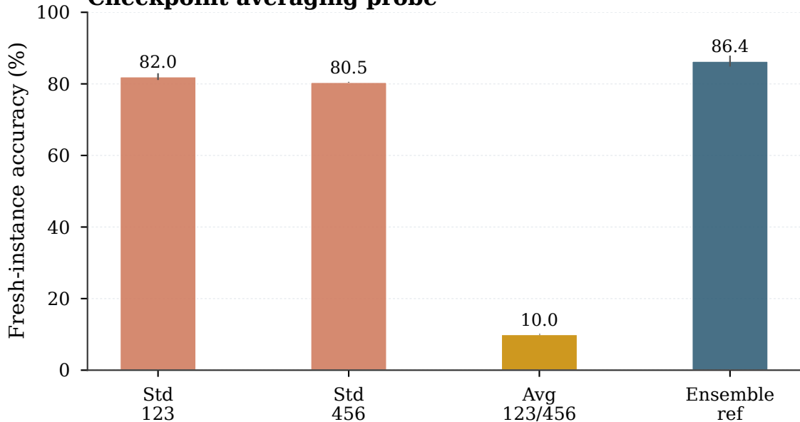
Checkpoint averaging probe
