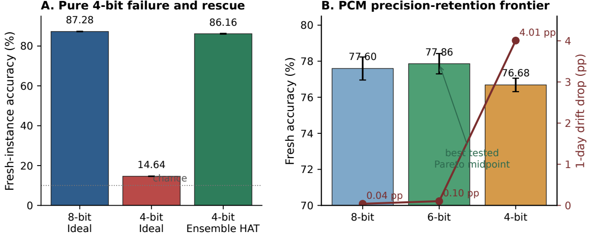
Figure 1: Paper-1 experimental spine. (A) AIHWKit IdealDevice is stable at 8-bit but collapses at 4-bit; Ensemble HAT rescues the 4-bit fresh-instance regime. (B) PCM UnitCell converges at 4/6/8-bit, but 4-bit drifts more over one day; 6-bit is the best observed precision-retention midpoint.
