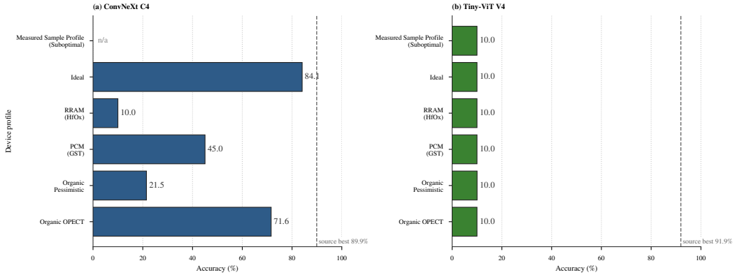
Figure 5: Zero-shot transfer across alternative device profiles. Bars report the accuracy of standard-HAT checkpoints when evaluated on literature-calibrated or measured alternative device profiles without profile-specific retraining. ConvNeXt C4 retains partial transfer on the OPECT and idealized profiles but degrades sharply on phase-change memory (PCM) and resistive random-access memory (RRAM), whereas Tiny-ViT V4 collapses to chance level (10.00%) across all shown alternatives. Dashed vertical lines mark the source-profile best accuracy, and unavailable architecture/profile combinations are labeled as n/a.
