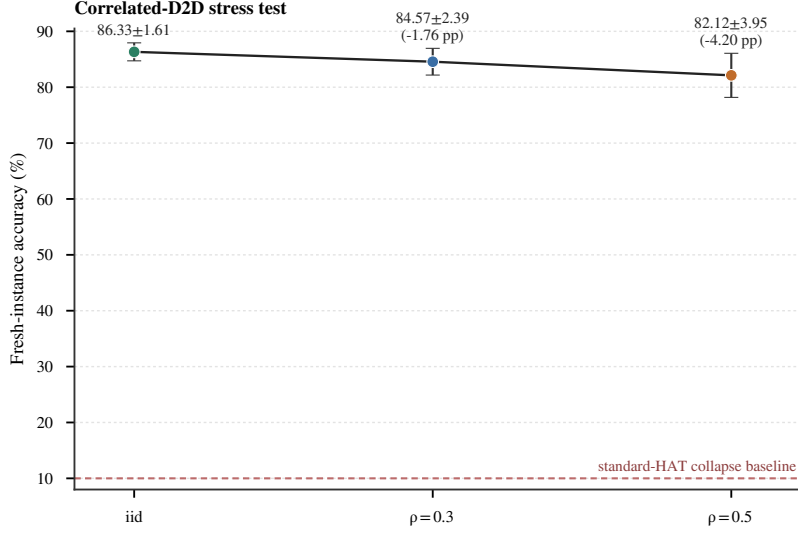
Figure 4.3: Fresh-instance robustness under spatially correlated D2D mismatch (reused from manuscript supplementary package, Fig. S5). Error bars show cross-instance standard deviation over 10 fresh arrays, with 5 Monte Carlo evaluations per array, for the canonical Tiny-ViT V4 Ensemble HAT checkpoint.
