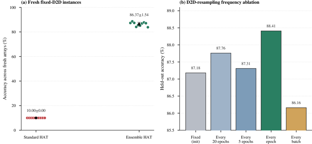
Figure 3.2: Fresh-instance robustness and D2D-resampling cadence ablation, reproduced from the manuscript supplementary package (Supplementary Figure S4). Left: standard HAT collapses to chance on every fresh array, whereas Ensemble HAT preserves robust accuracy. Right: held-out accuracy under different resampling cadences in a 50-epoch scan. Epoch-level resampling reaches 88.41 %, exceeding fixed-mask (87.18 %) and per-batch (86.16 %) controls.
