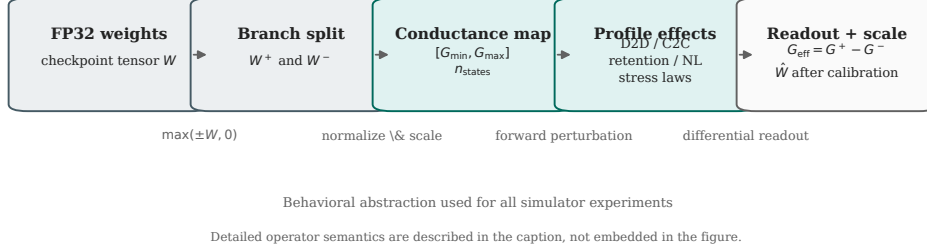
Figure 2.3: Differential-pair weight-to-conductance mapping reused from the manuscript. The digital weight tensor is split into positive and negative parts, normalized, mapped to the conductance window, quantized, and recombined as a differential effective weight.
