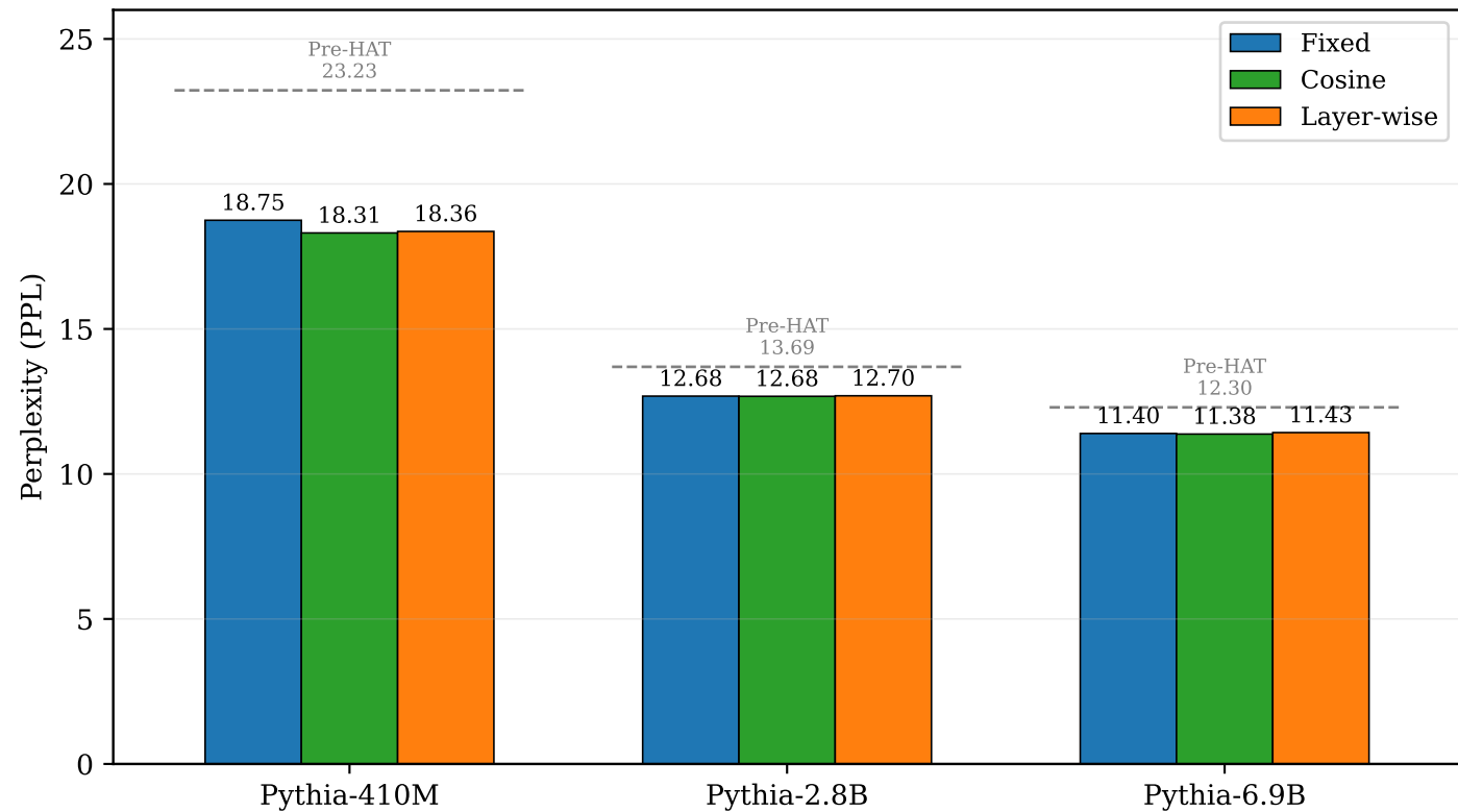
Adaptive Noise Schedule Comparison Across Model Scales
