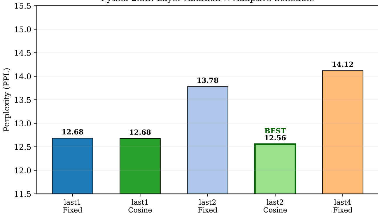
Pythia-2.8B: Layer Ablation × Adaptive Schedule
