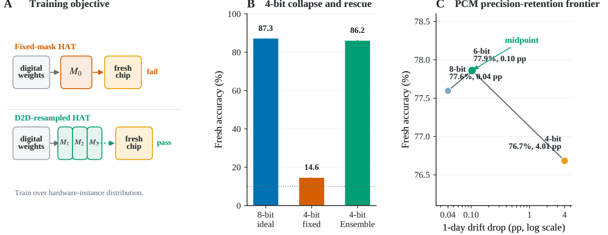
Figure 1: Paper-1 experimental spine. (A) Standard fixed-mask HAT optimizes one device instance, whereas Ensemble HAT trains over resampled D2D masks. (B) In the idealized AIHWKit baseline, 4-bit fresh-instance accuracy collapses while Ensemble HAT recovers it. (C) Under PCM UnitCell simulation, 4/6/8-bit models all train, but 4-bit has larger one-day drift and 6-bit is the best tested precision-retention midpoint.
