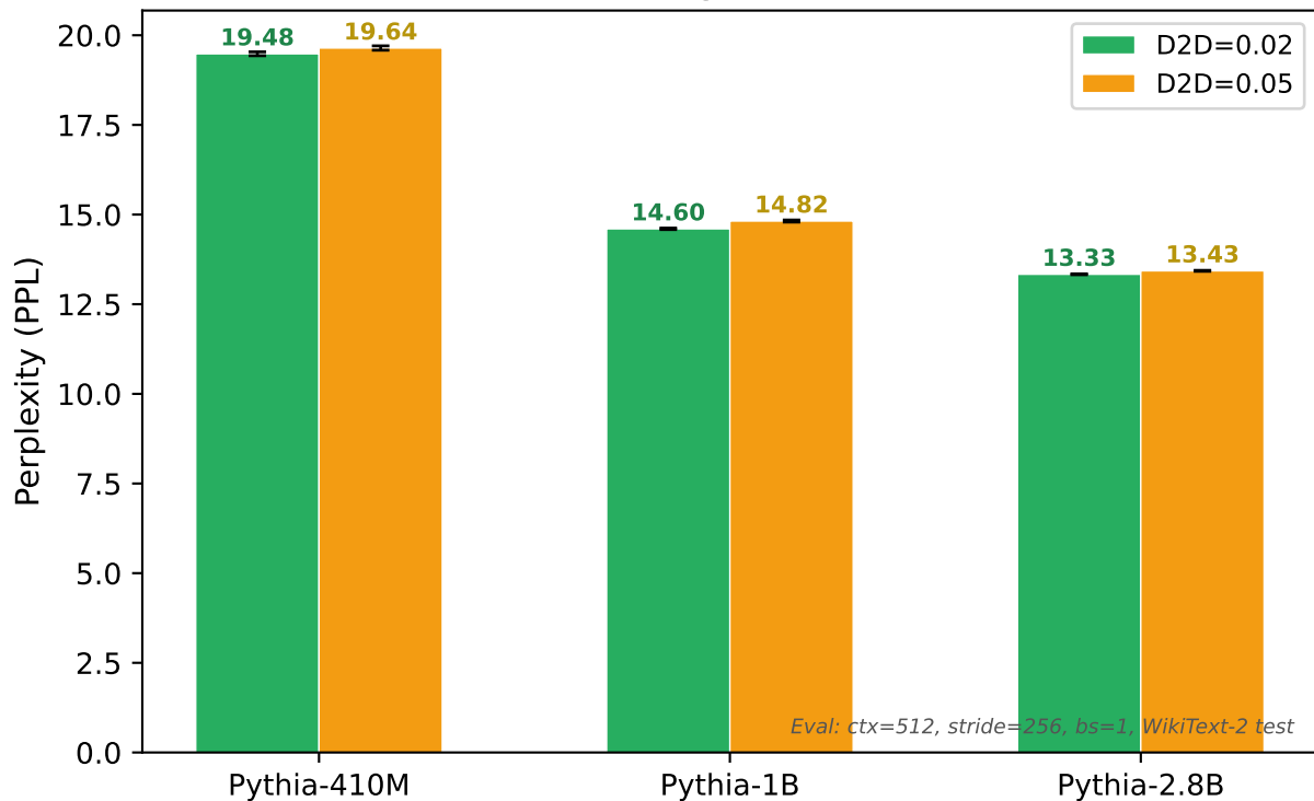
Scale Trend: Selective Terminal-Layer Analog KV (last1 config, mean \pm std)
