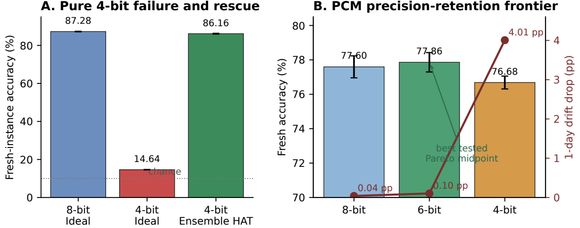
Figure 1: Paper-1 experimental spine. (A) The tested AIHWKit IdealDevice baseline is stable at 8-bit precision but collapses at 4-bit precision under fresh hardware instances; Ensemble HAT restores 4-bit fresh-instance accuracy by resampling D2D mismatch during training. (B) The tested PCM UnitCell regime separates trainability from retention: 4/6/8-bit models all converge, but 4-bit incurs a larger one-day drift drop while 6-bit gives the best observed precision-retention midpoint in the sweep. Error bars denote cross-seed standard deviation for the reported seed means.
