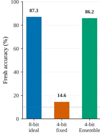
Figure 1: Paper-1 experimental spine. (A) Standard fixed-mask HAT optimizes one device instance, whereas Ensemble HAT trains over resampled D2D masks. (B) In the idealized AIHWKit baseline, 4-bit fresh-instance accuracy collapses while Ensemble HAT recovers it. (C) Under PCM UnitCell simulation, 4/6/8-bit models all train, but 4-bit has larger one-day drift and 6-bit is the best tested precision-retention midpoint.
