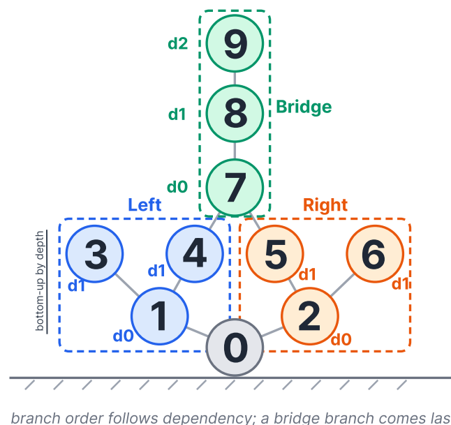
(e) Step 4: Group by branch and depth
