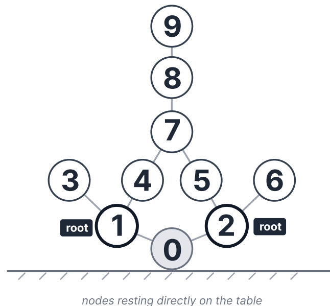
(b) Step 1: Identify root nodes
