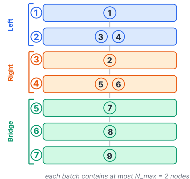
(f) Step 5: Cut into ordered batches
