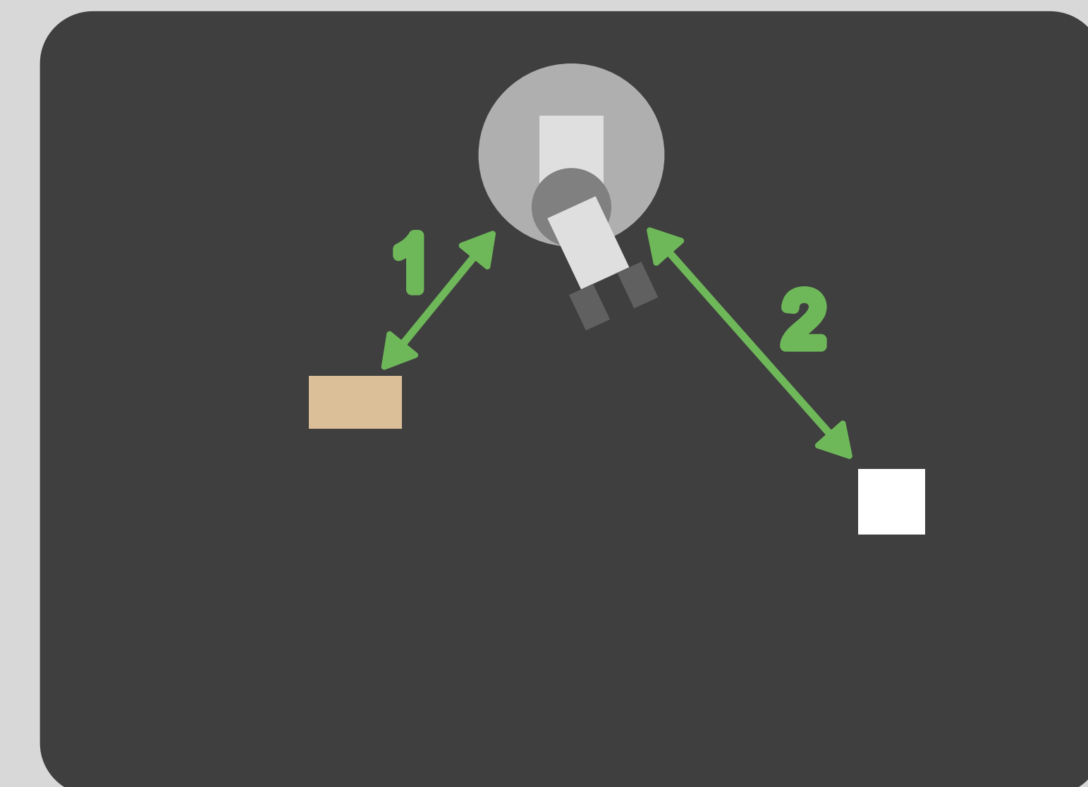
0.1.2 Manipulability-Aware Ordering
