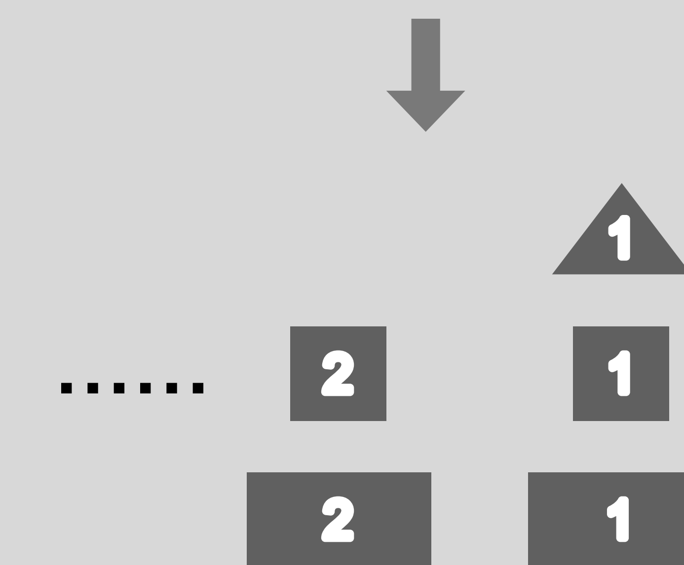
0.2.2 Manipulability-Ranked Candidates
