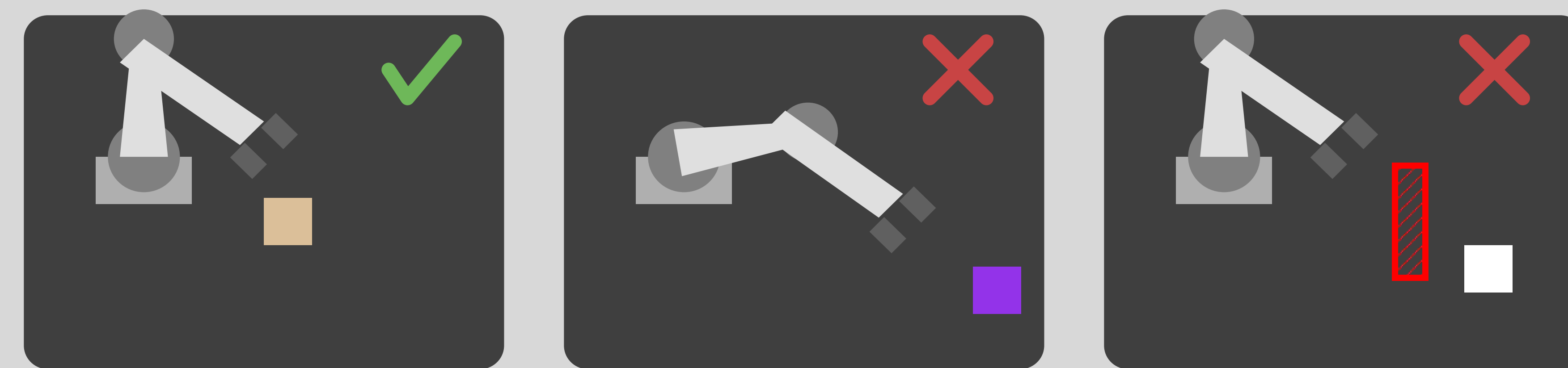
0.1.1 Reachability Screening
