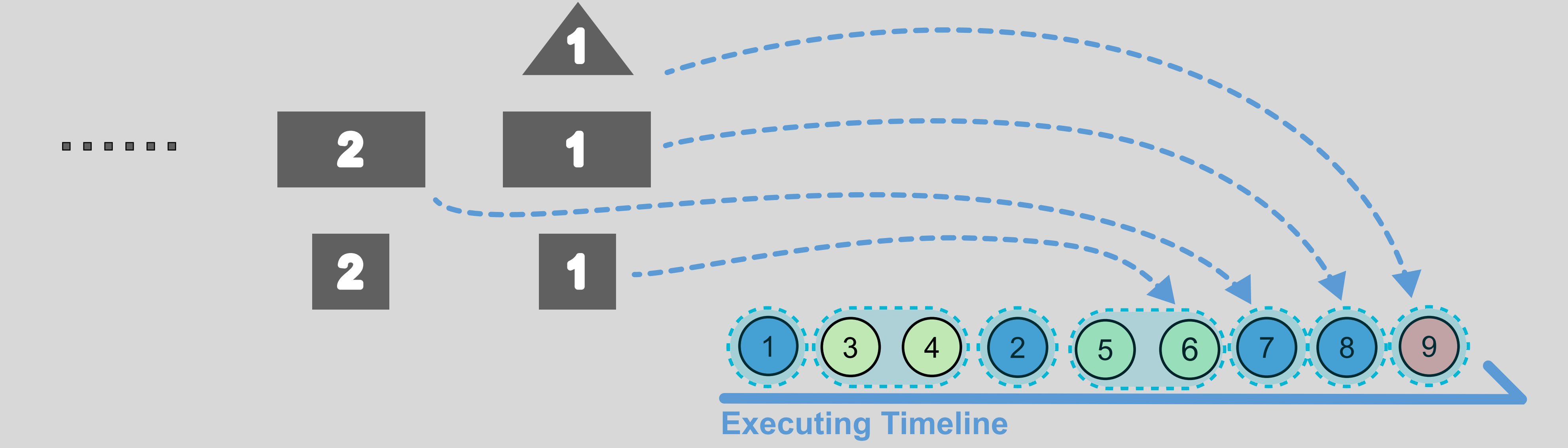
Execution-Order Embedding
