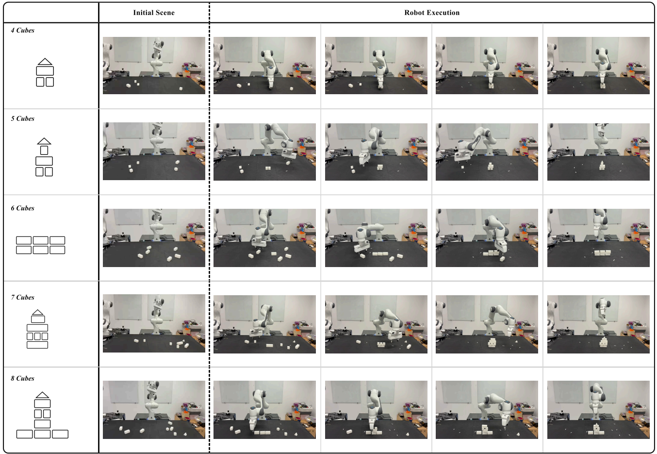
Fig. 5. Representative real-robot execution: initial scene and execution-sequence photos for cube-stacking assemblies of 4 to 8 cubes on the physical Franka Panda platform. ZZ: change this figure
