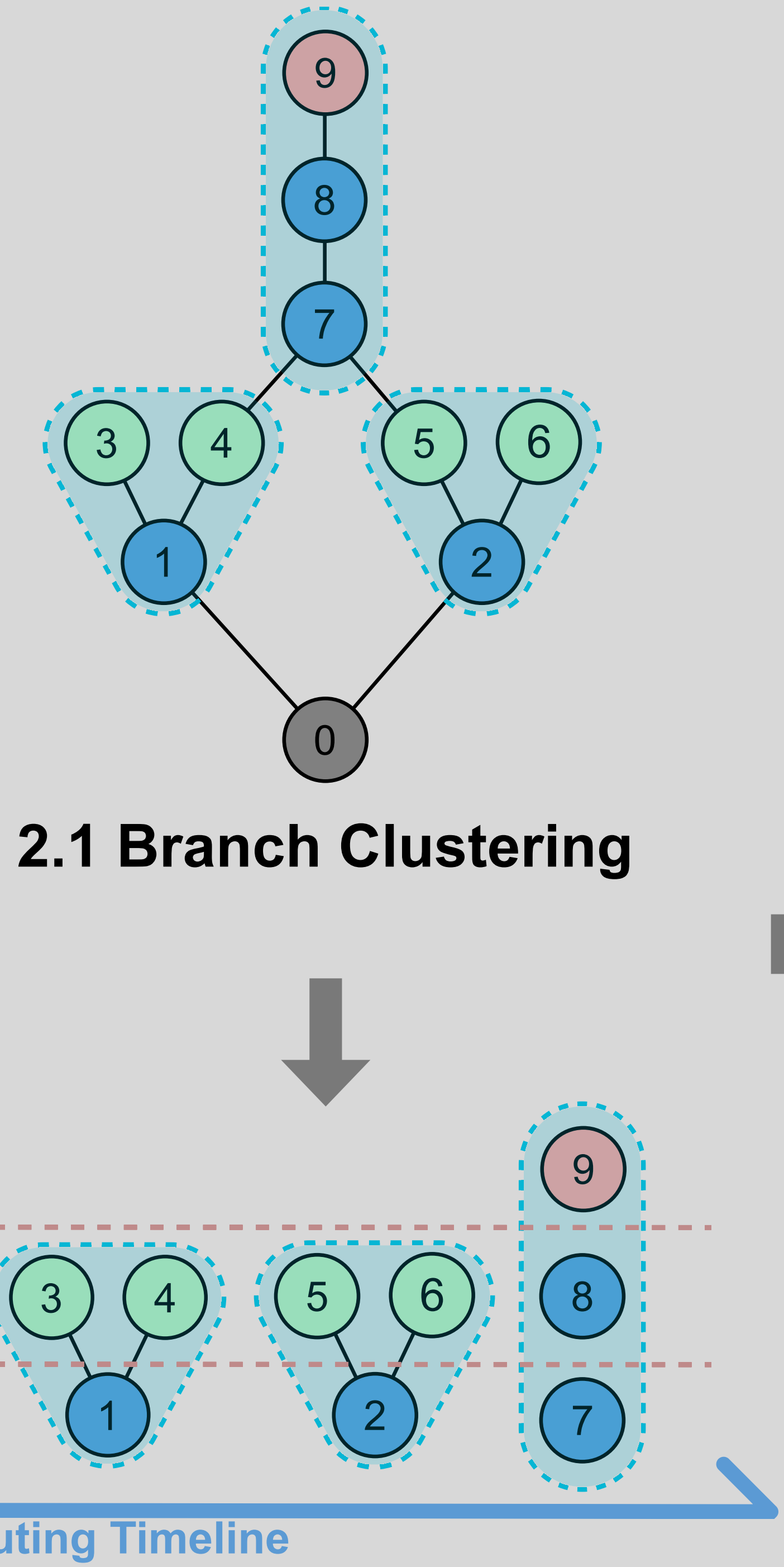
2. Two-Level Clustering
