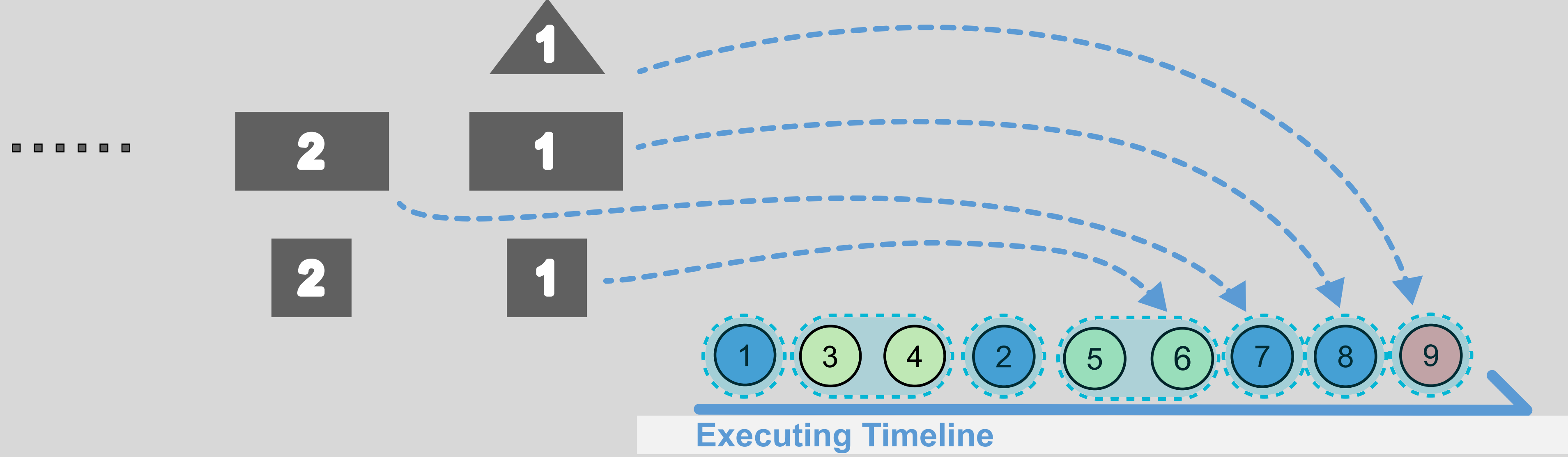
Execution-Order Embedding
