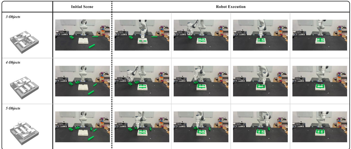
Fig. 7. Representative real-robot execution: initial scene and execution-sequence photos for FMB assemblies of 3 to 5 objects on the physical Franka Panda platform. ZZ: change this figure
