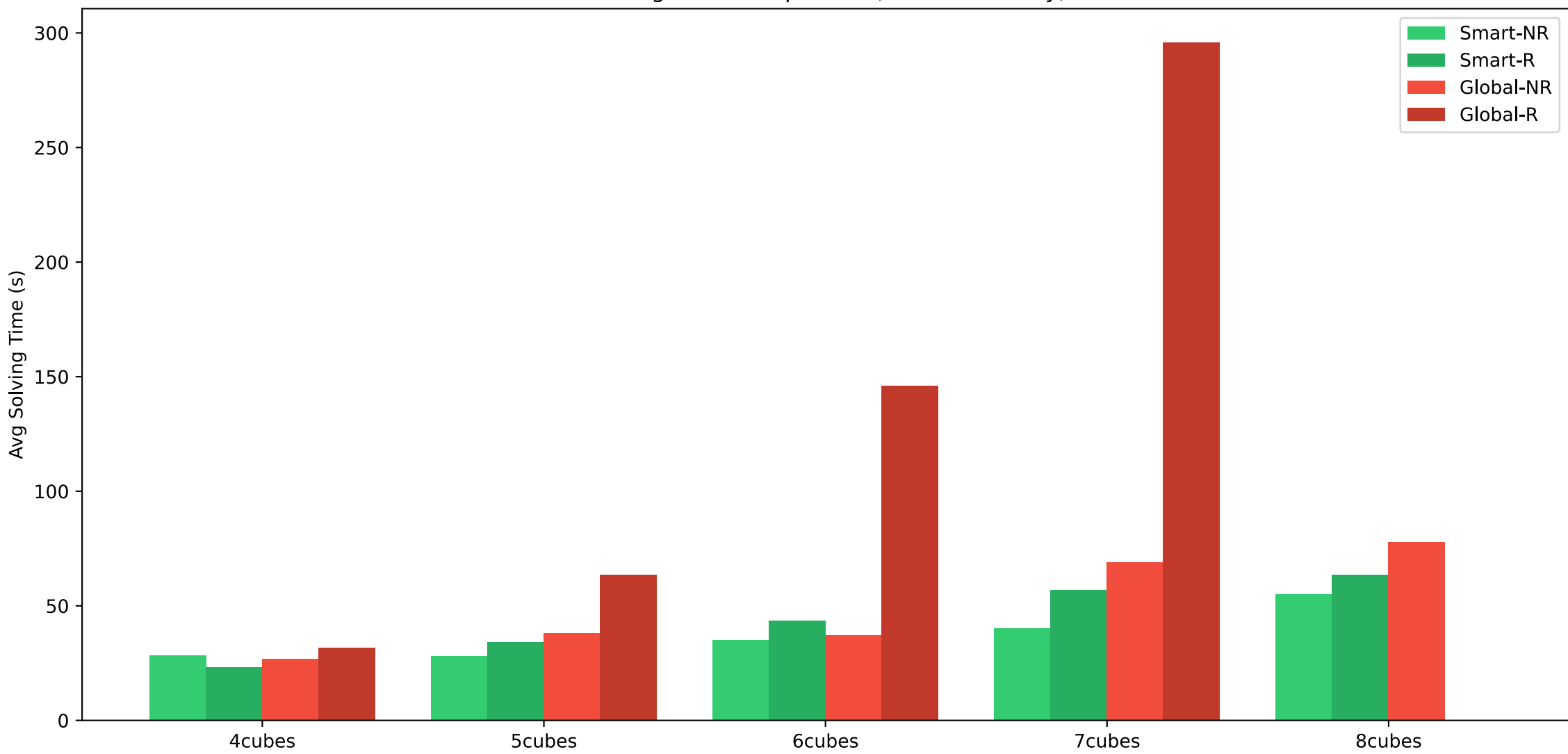
Solving Time Comparison (Successful Only)
