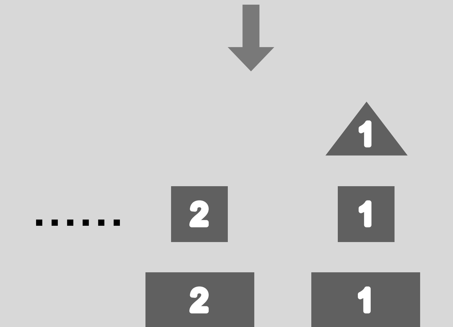
0.2.2 Ordered by Euclidean distance
