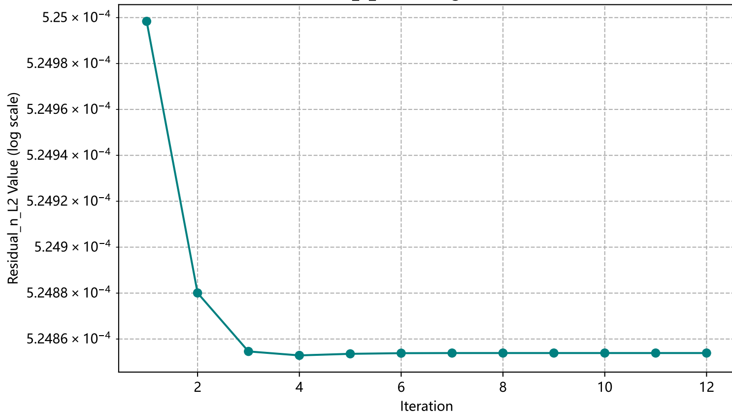
Residual_n_L2 Convergence (Va=0.3)
